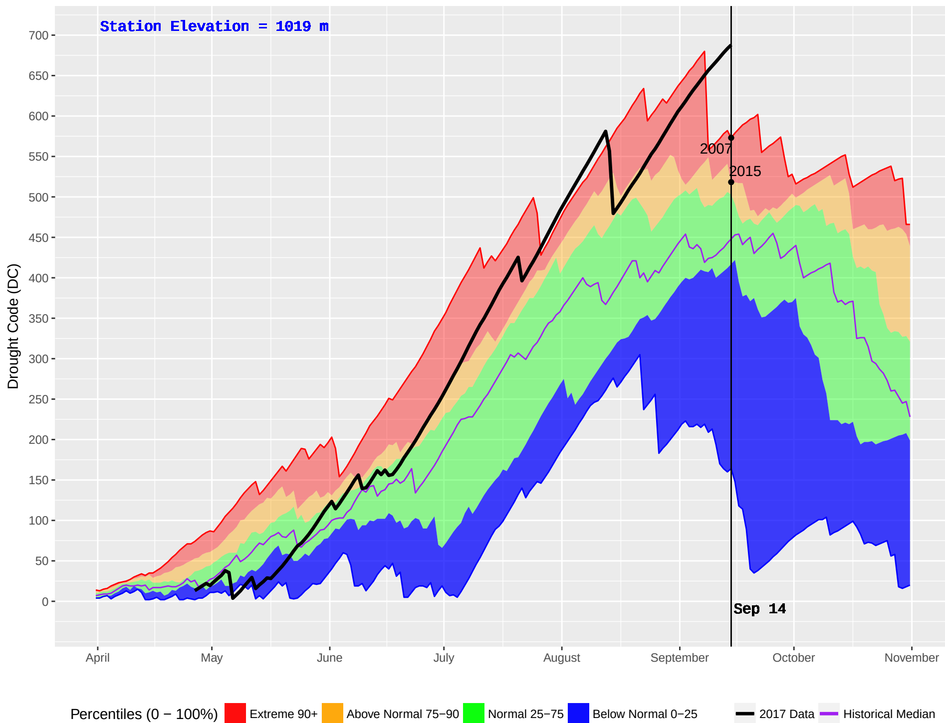
POWDER CREEK (380) : Historical (2001–2016) and Current (2017) Noon Drought Code (DC)
